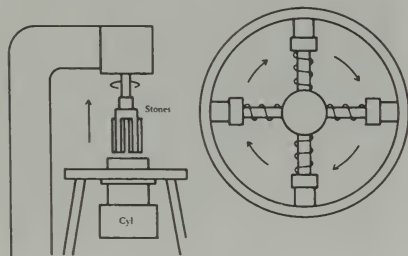
FIGURE 10-21. Cylinder honing.
